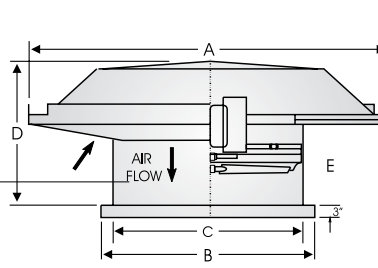
Model HRSB Supply Belt Drive Model HRSD Supply Direct Dive
